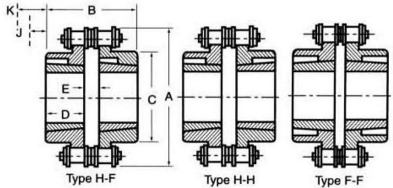
Taper-lock Chain Coupling
