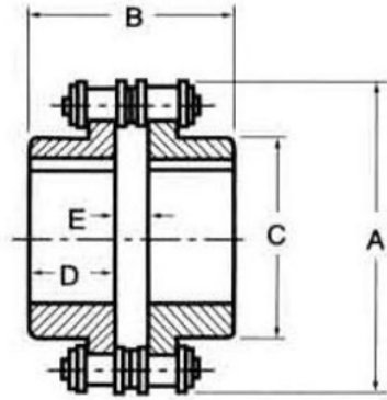
Straight Bore Chain Coupling
