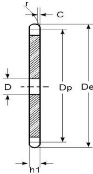
CONVEYOR SERIES-CARRIER ROLLER DUPLEX PITCH-2080/C2080
